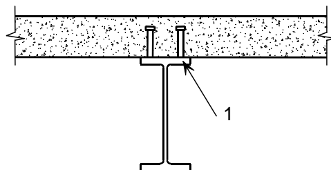
1 compression flange
